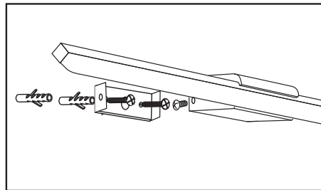
Para pared/wall fixing
